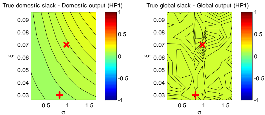
FIGURE E12. Correlations of variables as a function of the parameters of openness Period 1 and Period 2 (benchmark) parameters are denoted by '+' and 'x', respectively.
